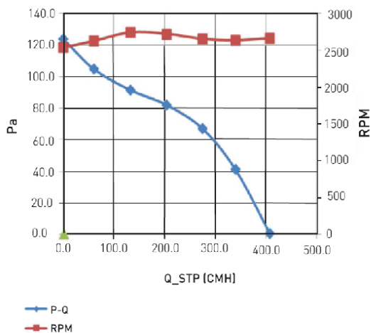
Fan Pressure Curve Diagram
