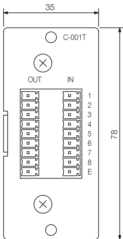
Front View
