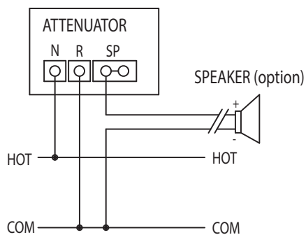
2-WIRE SYSTEM
