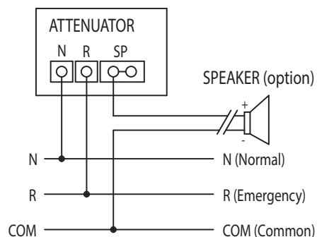
3-WIRE SYSTEM
