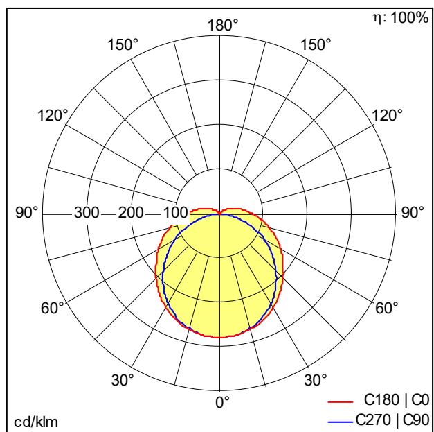
TE_LUCY_1200_LED_IP66_4000_840.idt
