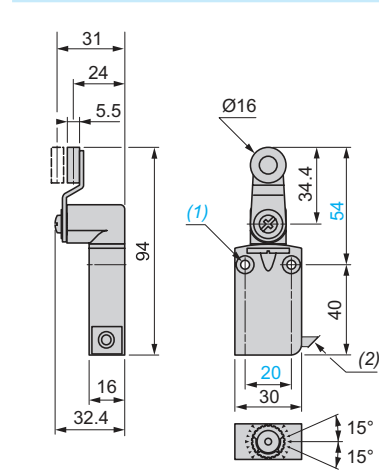
XCMD2115M12 /116M12 /117M12 XCMD2115C12 /116C12 /117C12
