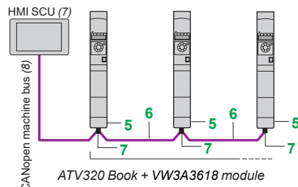
Example of connection to the CANopen machine bus via SUB-D connector
