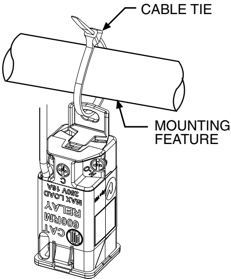
Figure 5: Cable Tie Mounting Illustration
