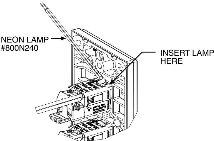
Figure 4: Installation Of Neon Indicator
