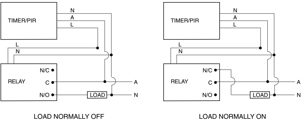
Figure 1: Relay Wiring Diagram
