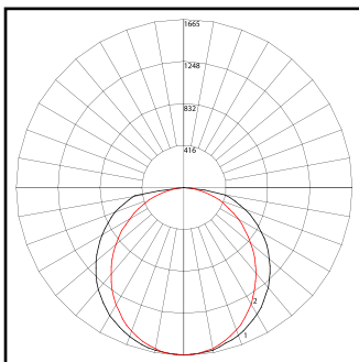
Typical Polar distribution Standard Fittings
