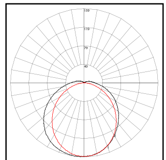
Typical Polar distribution 5ft Emergency
