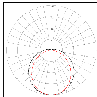
Typical Polar distribution 4ft Emergency
