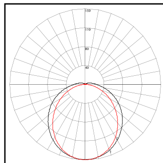
Typical Polar distribution 2ft Emergency
