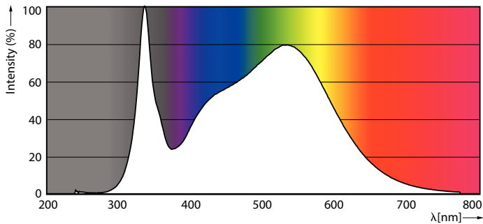
Spectral Power Distribution Colour - CorePro LEDtube 1200mm 18W 5CCT T8 AU
