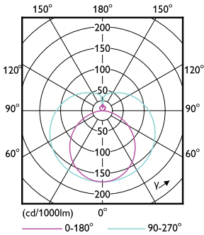
Light Distribution Diagram - CorePro LEDtube 1200mm 18W 5CCT T8 AU
