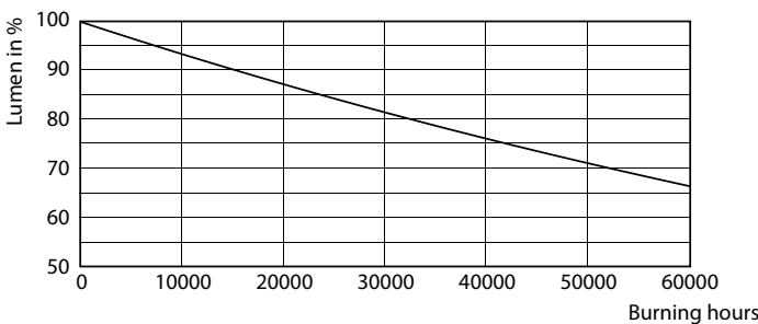
Lumen Maintenance Diagram - CorePro LEDtube 1200mm 18W 5CCT T8 AU
