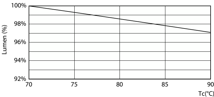
Lumen Maintenance Diagram - CorePro LEDtube 1200mm 18W 5CCT T8 AU
