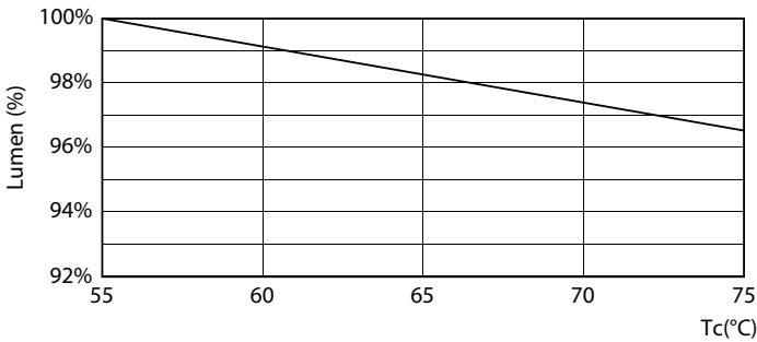
Lumen Maintenance Diagram - CorePro LEDtube 1200mm HE 18W 840 T5AU
