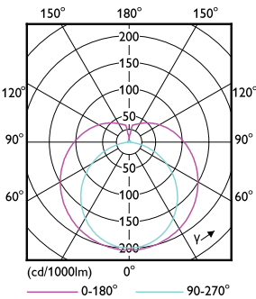
Light Distribution Diagram - CorePro LEDtube 1200mm HE 18W 840 T5AU
