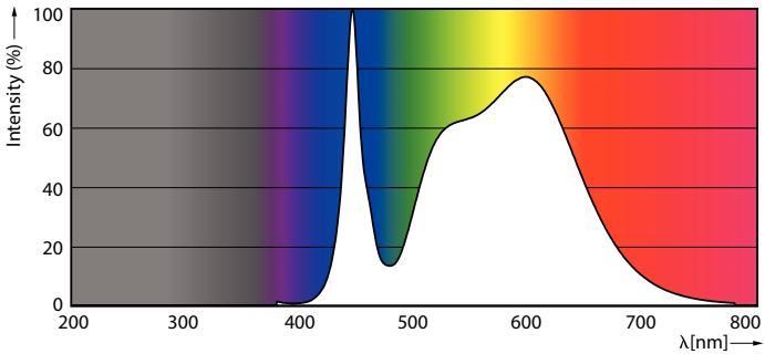
Spectral Power Distribution Colour - CorePro LEDtube 1200mm HE 18W 840 T5AU
