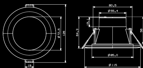
KING D90 Dimensions
