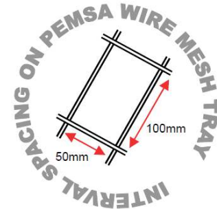
Rejiband 35 Wire mesh tray
