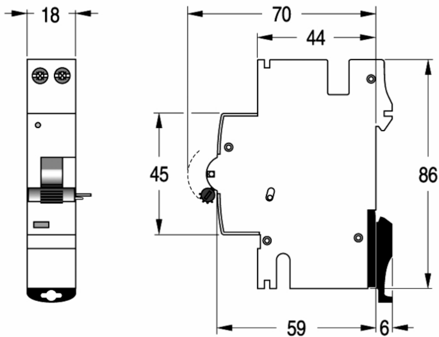
Dimension Diagram
