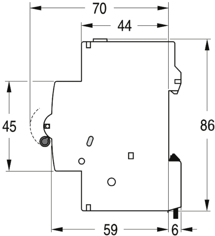
Dimension Diagram
