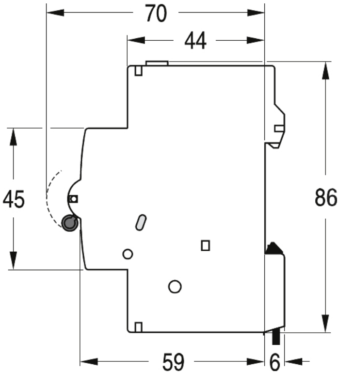
Dimension Diagram
