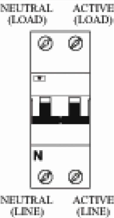
Connection / Wiring Diagram
