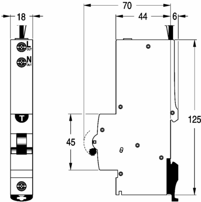
Dimension Diagram
