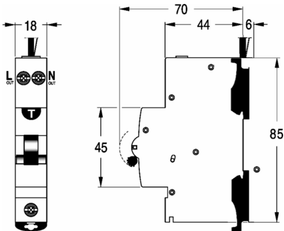
Dimension Diagram
