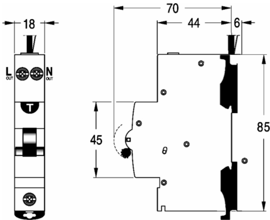
Dimension Diagram
