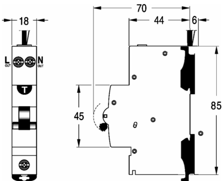
Dimension Diagram
