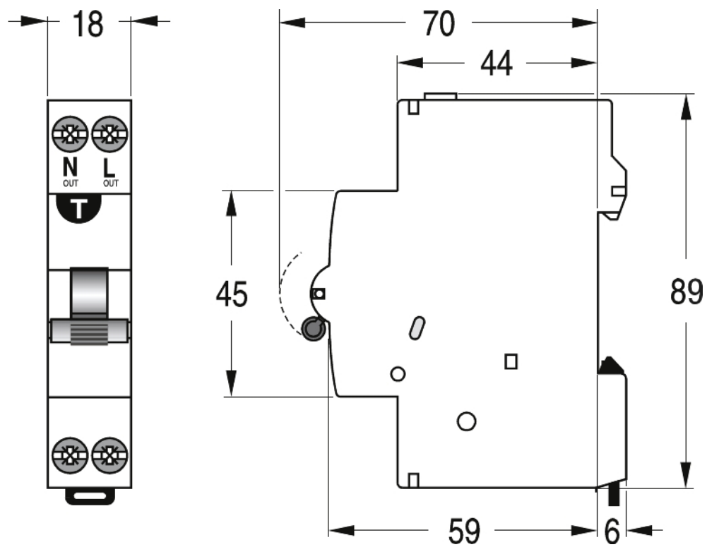
Dimension Diagram
