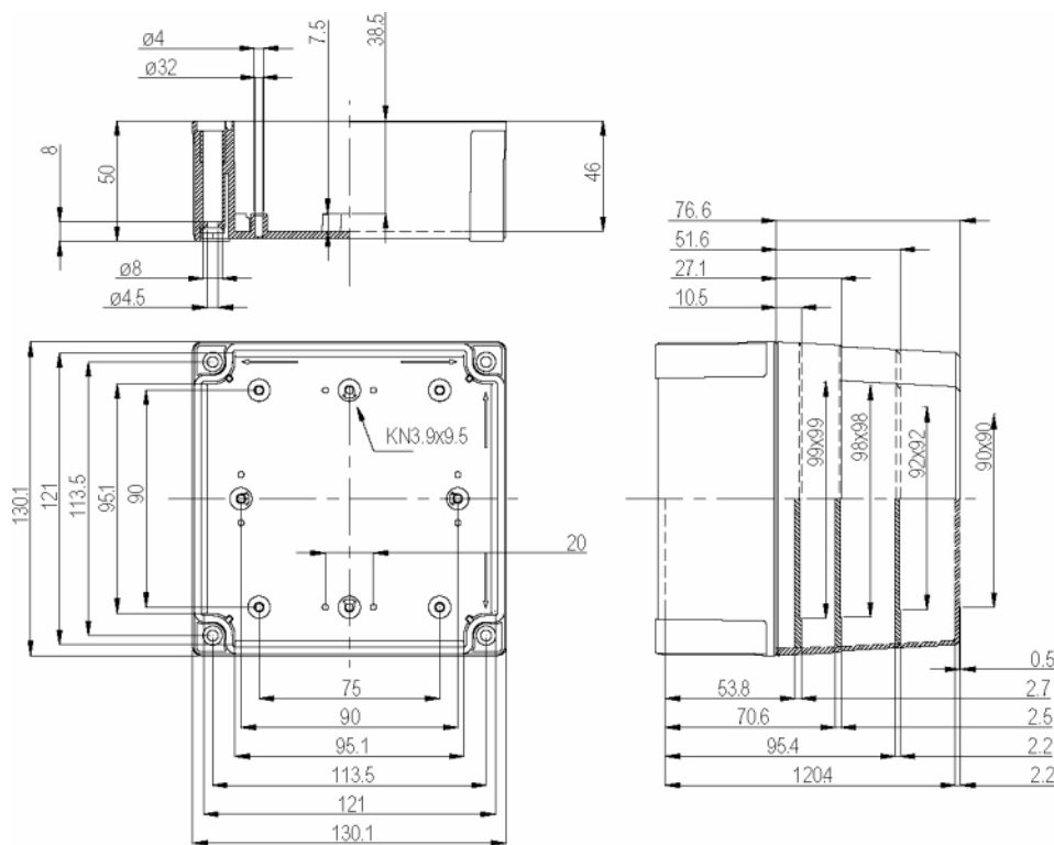
Dimension Diagram
