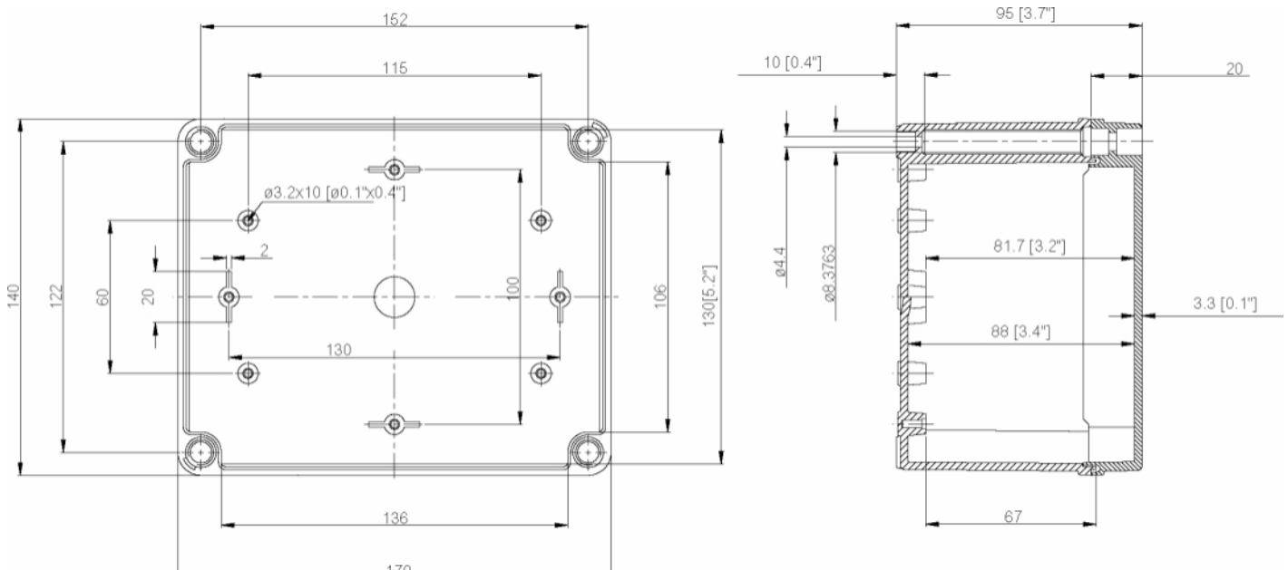
Dimension Diagram
