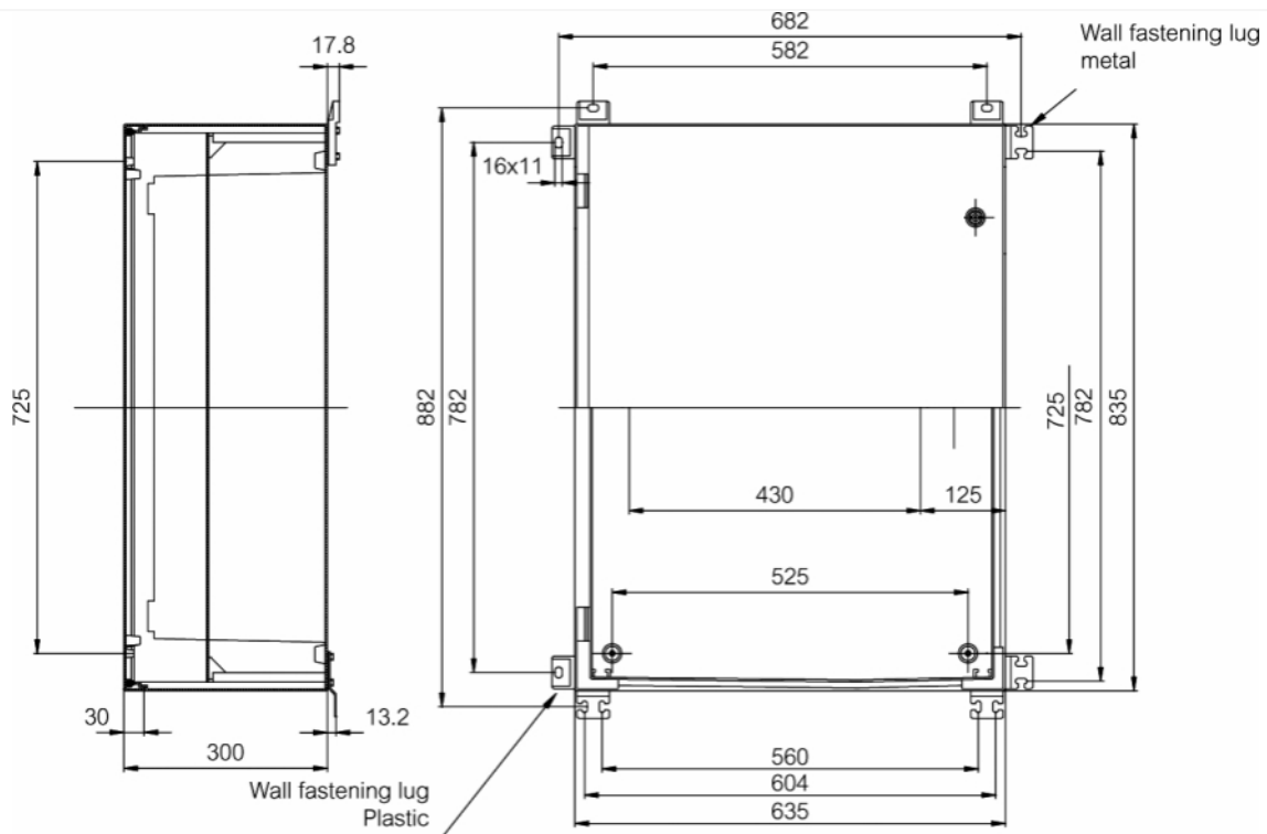
Dimension Diagram
