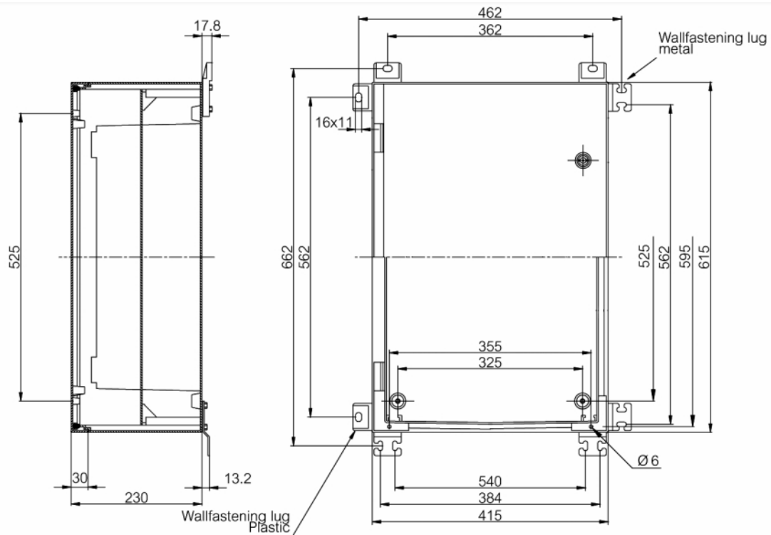
Dimension Diagram
