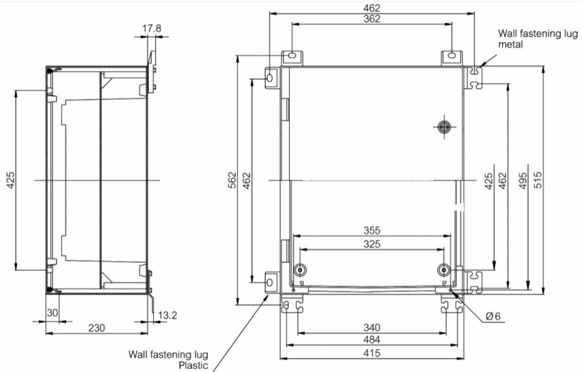
Dimension Diagram
