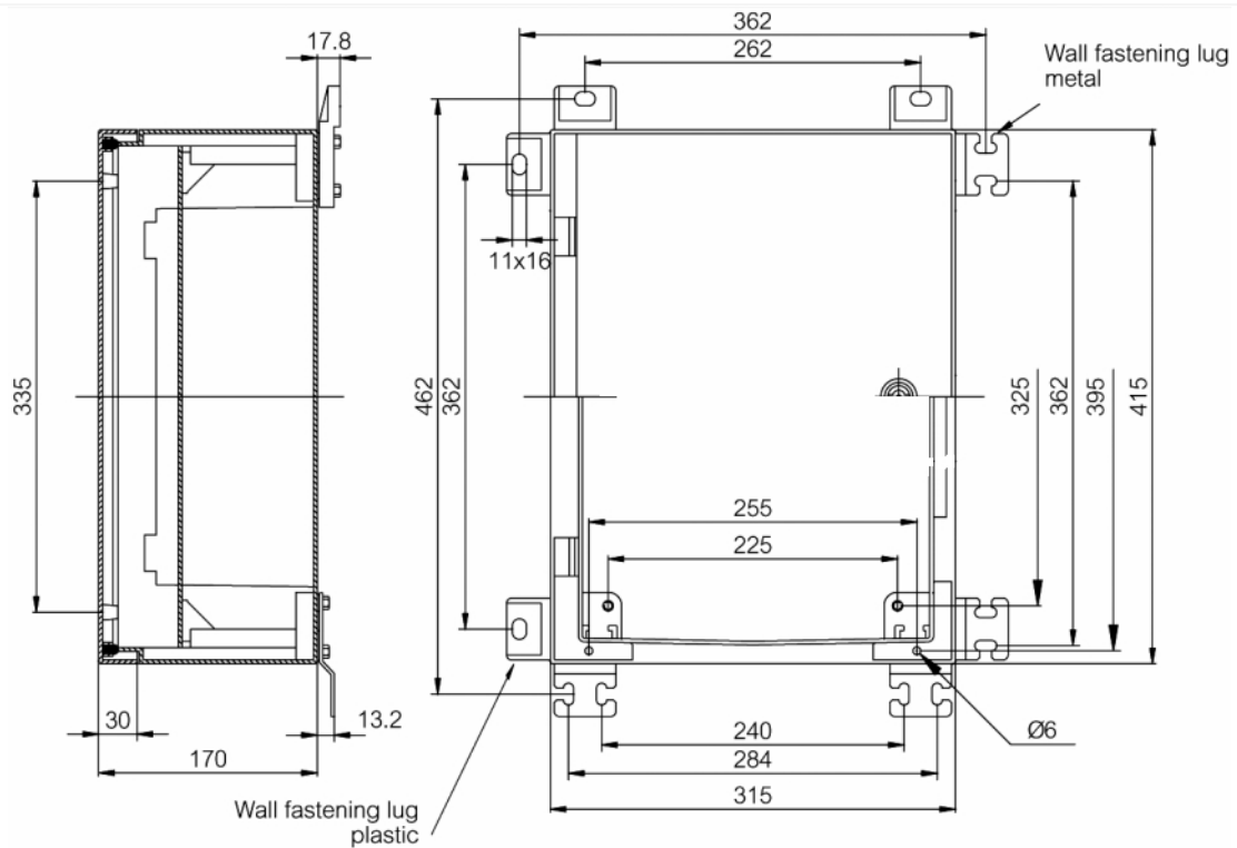
Dimension Diagram
