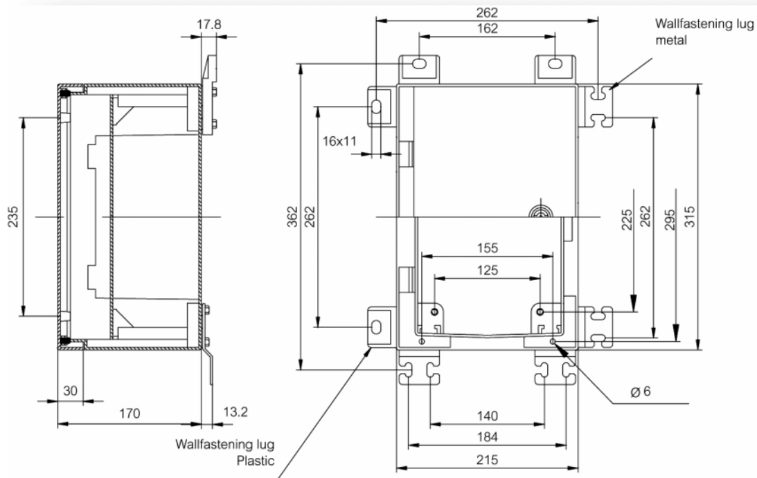
Dimension Diagram
