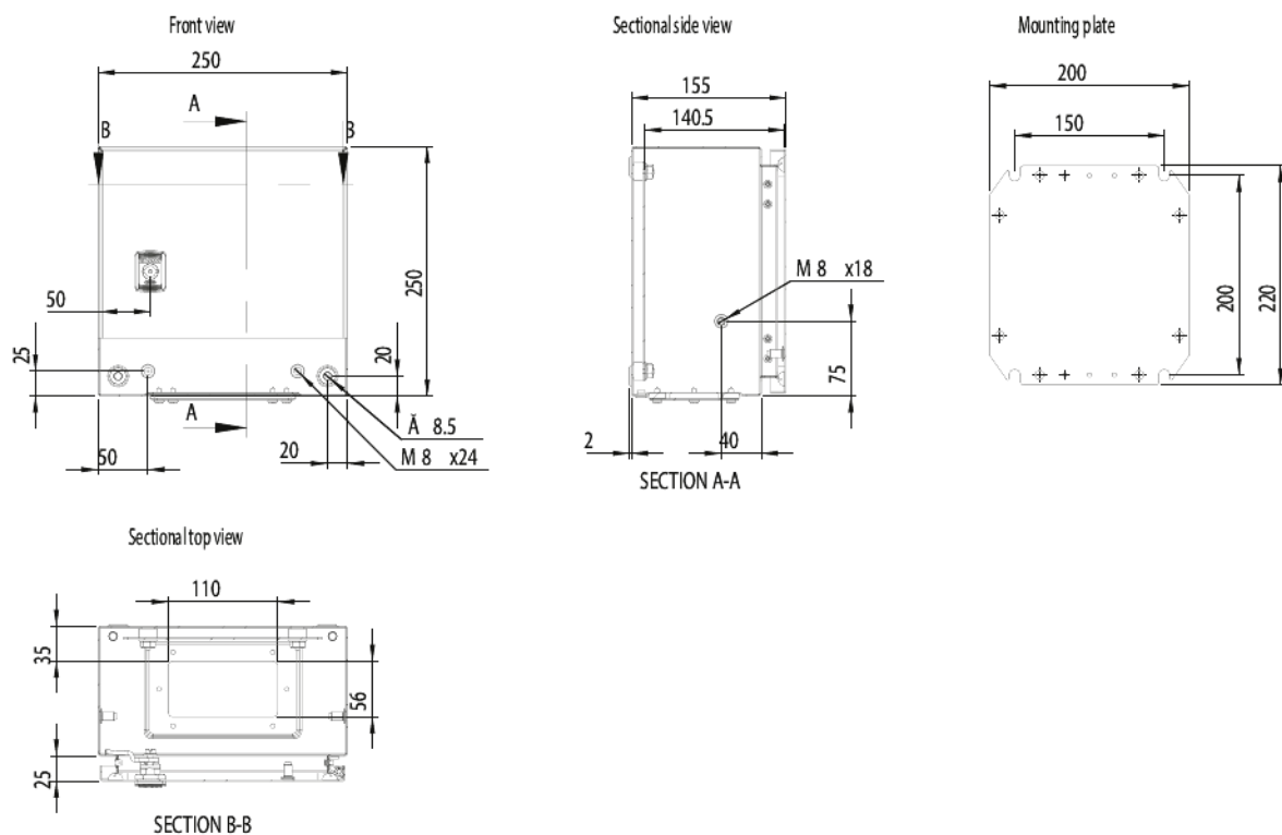
Dimension Diagram
