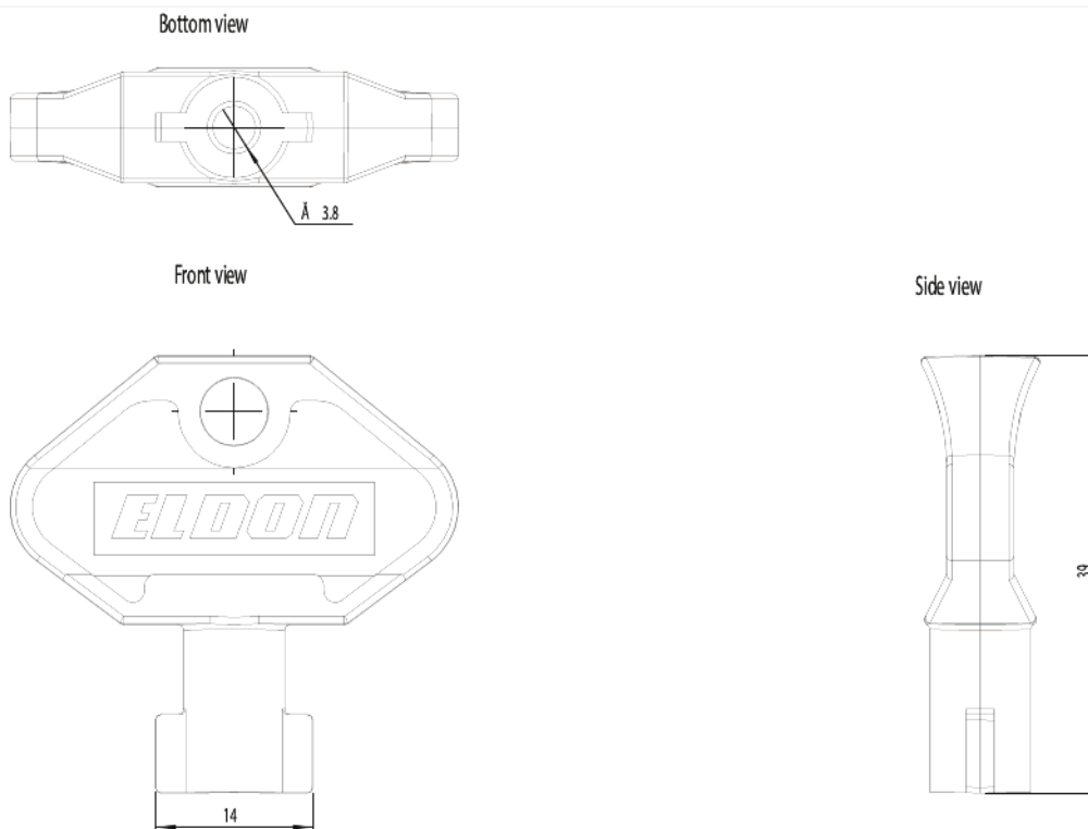
Dimension Diagram
