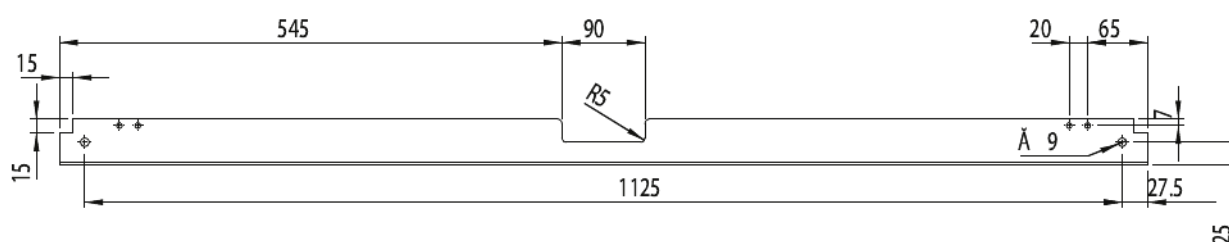
Dimension Diagram
