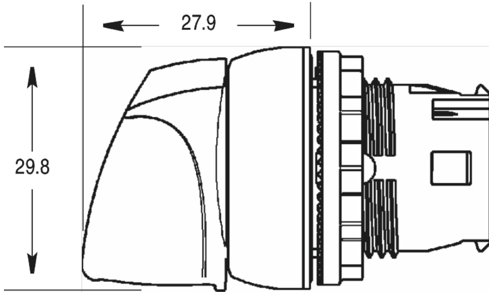
Dimension Diagram
