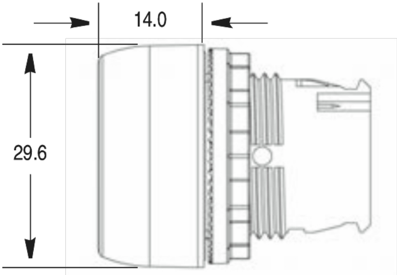
Dimension Diagram
