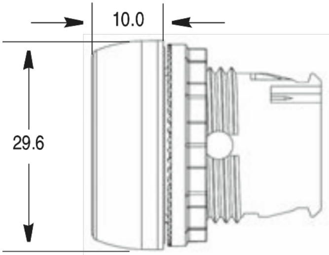
Dimension Diagram
