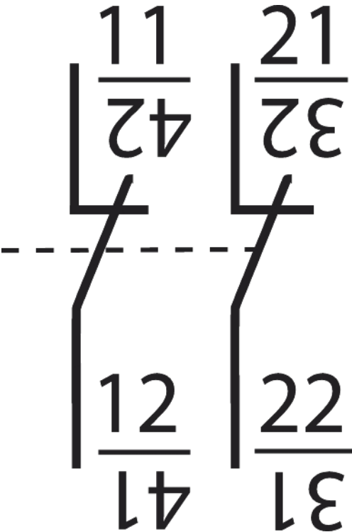
Connection / Wiring Diagram
