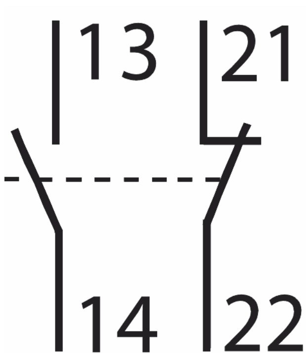
Connection / Wiring Diagram
