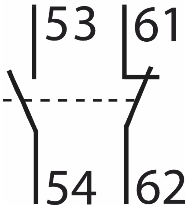
Connection / Wiring Diagram
