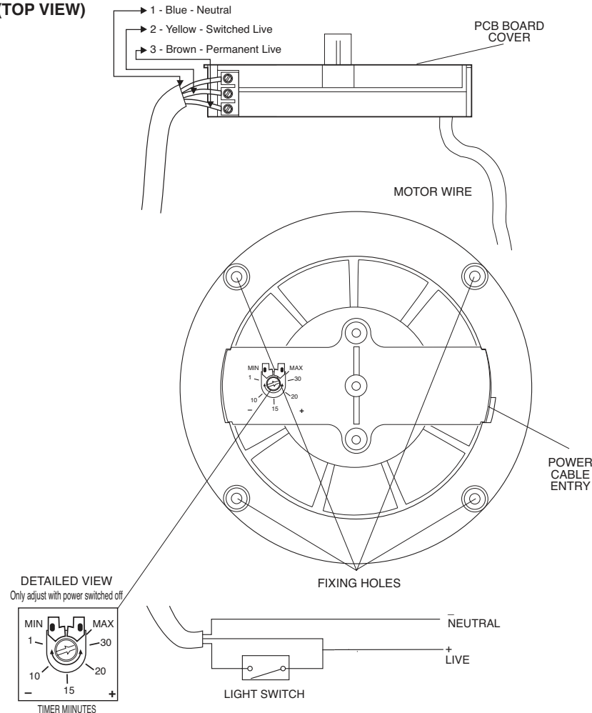
DIAGRAM 2 TIMER MODEL
