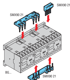
Connections for star-delta assembly
