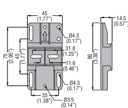
BFX89 01 fixing base
