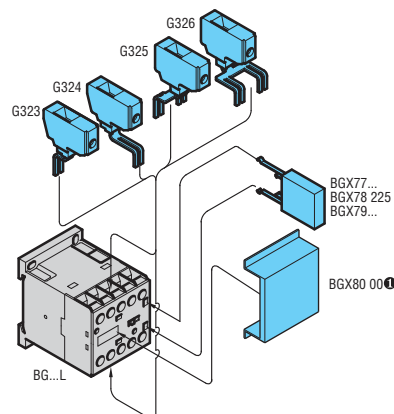
Combinations: Mounting position on BG...L mini-contactors
