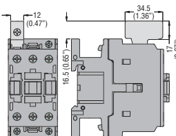
G232 terminal 1-pole
