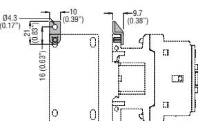
BFX89 02 fixing bracket
