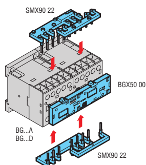
Connections for reversing contactor assembly
