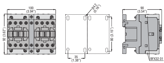
Rigid connecting kits BFX32 01
