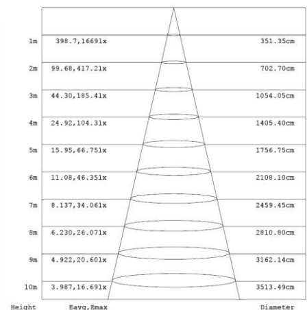
Diagram for RDL50CCT36012F-01 in 6500K. Other diagrams available on
