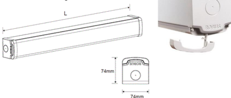
Dimension Diagram
