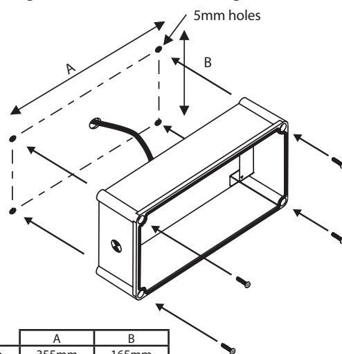
Mounting holes for direct wall mounting
