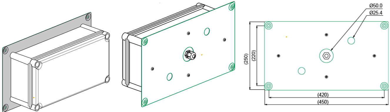
24m - wall bracket
