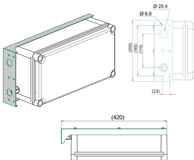
24m - side bracket
