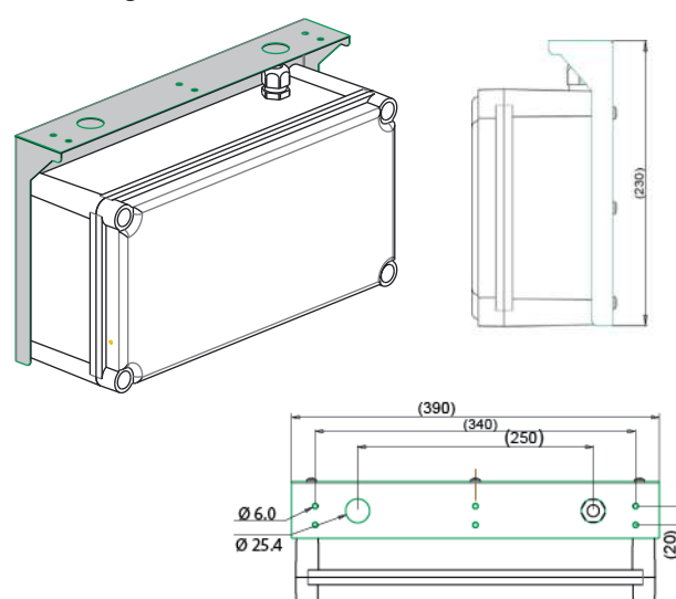
24m - ceiling bracket
