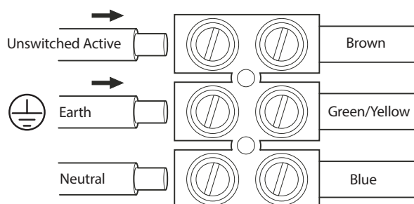
Main supply connection
