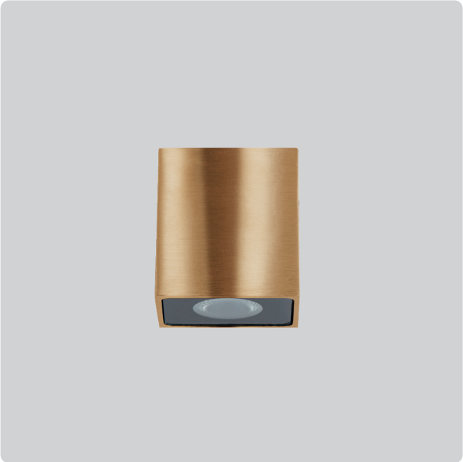
X983 Block Dimensions W40 x H45 x D45mm Beam 42° Watts 1.5W Lumens 110lm
