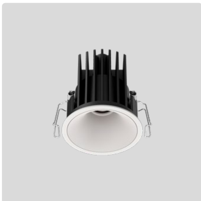
R536 Medium Fixed Dimensions D83 x H85mm Cut Out Ø 76mm Watts 14W Lumens <1065lm Beam 40°
