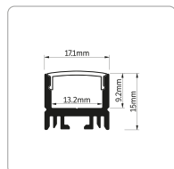
XS1715 Medium Narrow with Heat Sink
