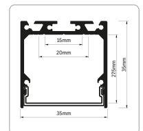
XS3535 Large Standard
