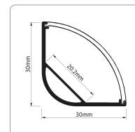
XS3030 Corner Mount
