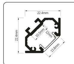
XS2222 Corner Mount Multi-Purpose Angled Surface Mount installation for directional applications.
