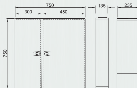
3 Size 3 750mm x 750mm 750 x 750 SIZE
