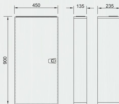
2 Size 2 450mm x 900mm 450 x 900 SIZE
