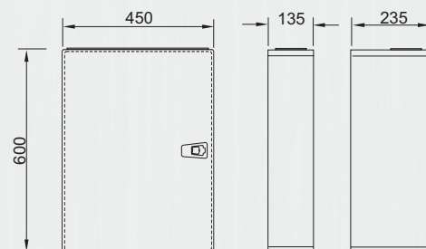
1 Size 1 450mm x 600mm 450 x 600 SIZE
