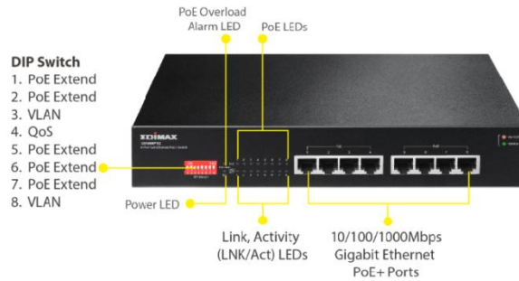
Front Panel
