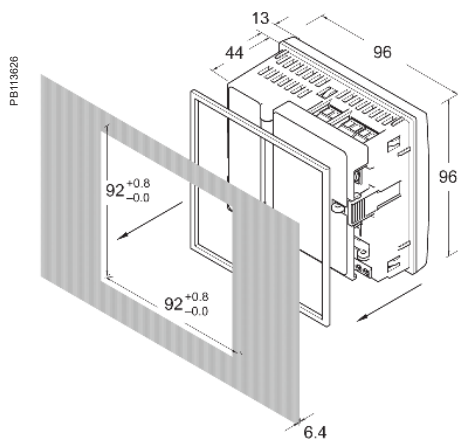
Dimensions PM5350IB
