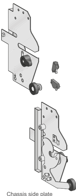
Chassis side plate
