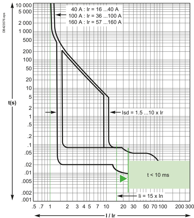
MicroLogic 2.2, 4.2 - 40... 160 A
