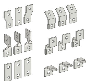
Terminal extensions
