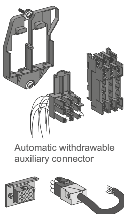
Manual auxiliary connector
