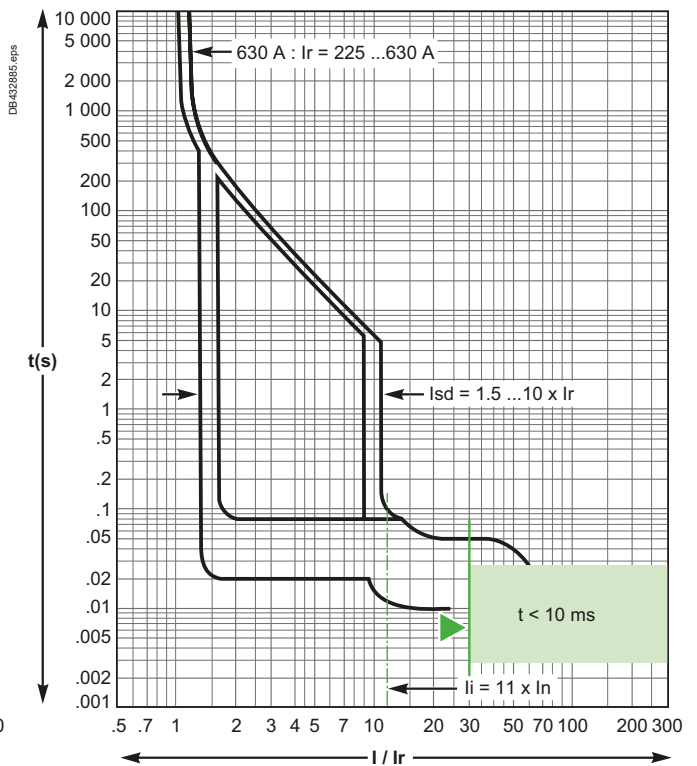
MicroLogic 2.3, 4.3 - 630 A
