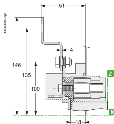
NSX100 to 250
