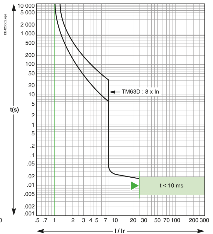
TM63D
