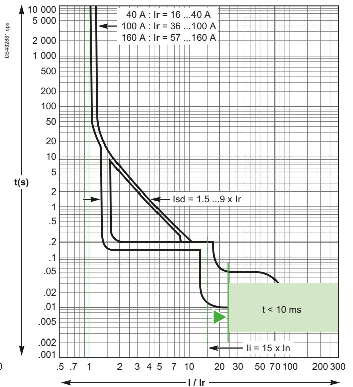
MicroLogic 2.2, 4.2 - 250 A
