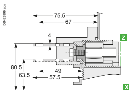
NSX100 to 250
